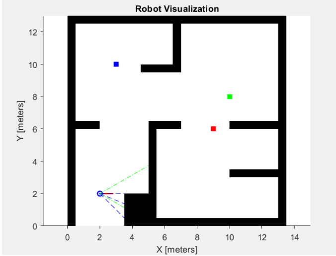
Fig. 4 The initial position of the mobile robot in first scenario.
