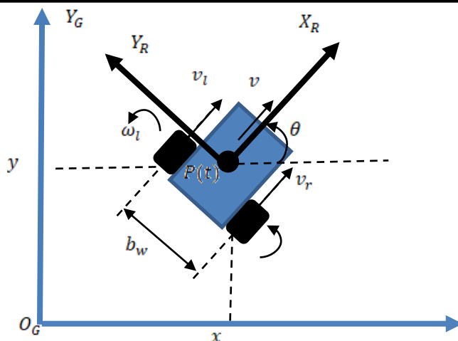
Fig.1. Schematic diagram of differential drive mobile robot.
