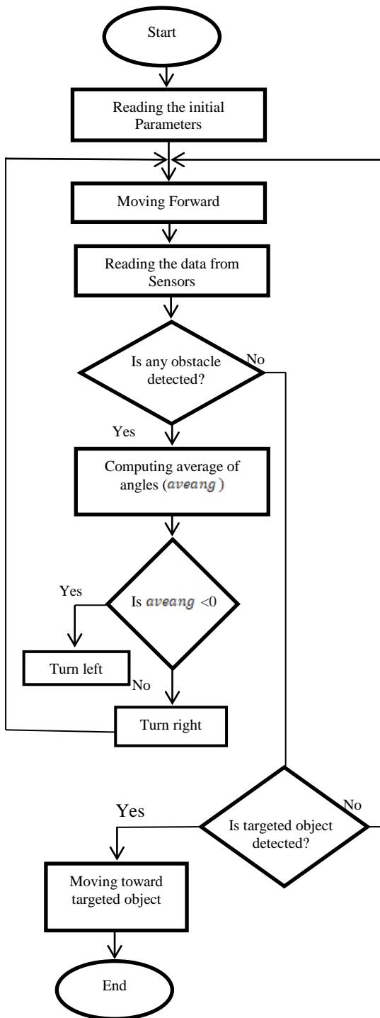
Fig.3. Flowchart of finding object and obstacle avoidance algorithm.
