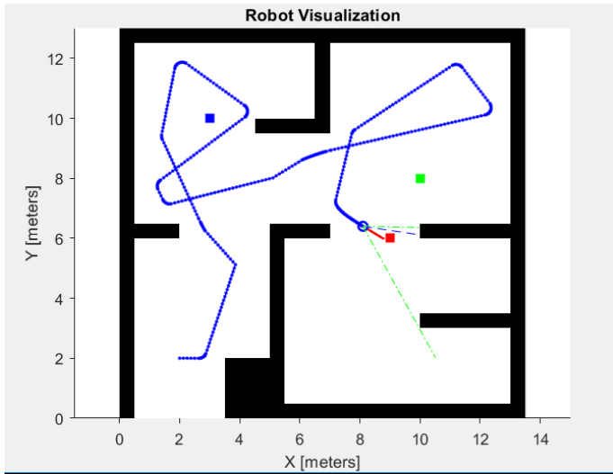
Fig. 5 The searching path of the mobile robot of the first scenario.
