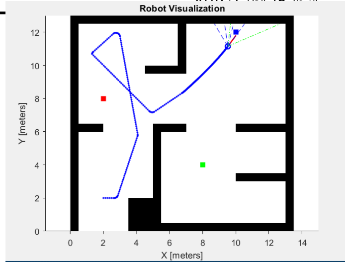
Fig. 7 The searching path of the mobile robot of the second scenario.
