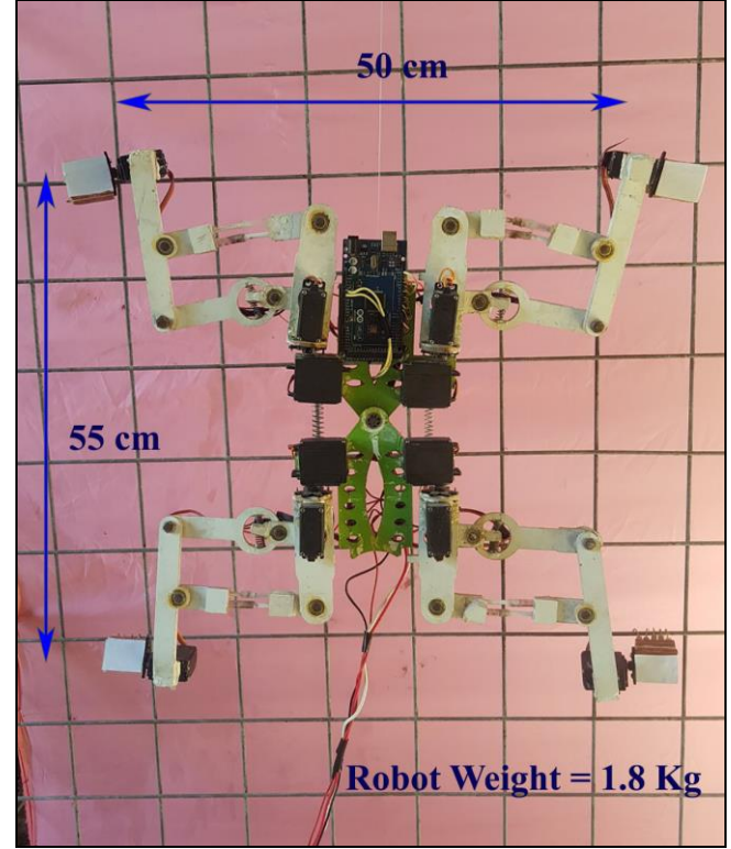
Fig. 3 climbing robot prototype climbing a mesh wall
