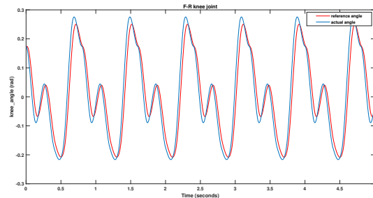
Fig. 14. Reference angle and actual angle comparison for knee joint.
