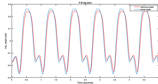
Fig. 20. Reference angle and actual angle comparison for hip joint.
