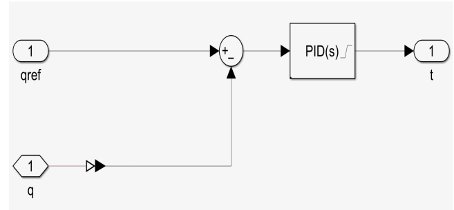
Fig. 6. PID controller system
