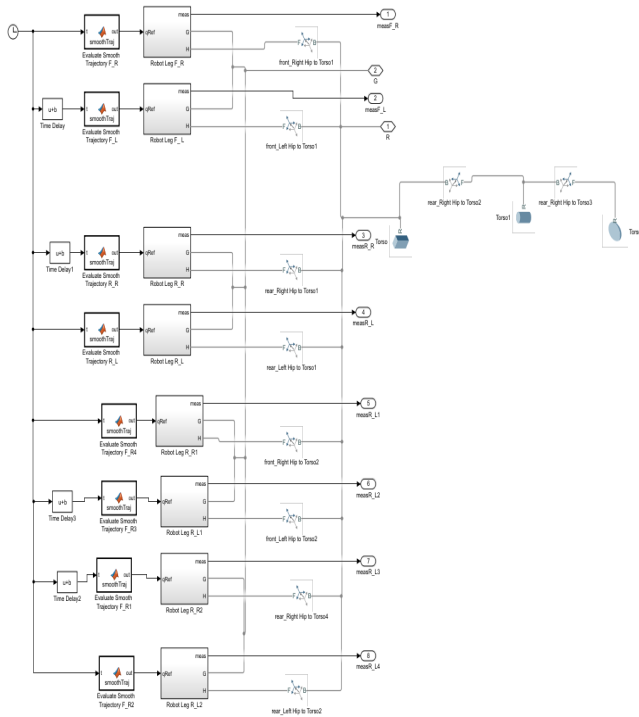
Fig. 3. robot sub-system that contain eight legs
