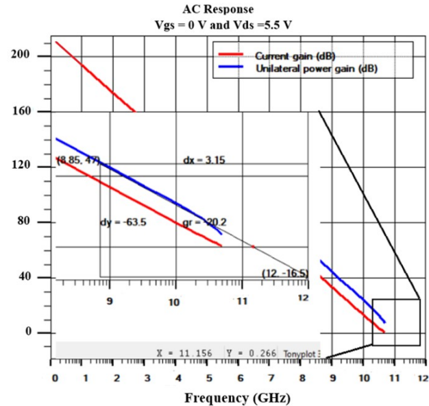
Fig. 10. Extraction of Maximum Frequency ( f_{max} ).
