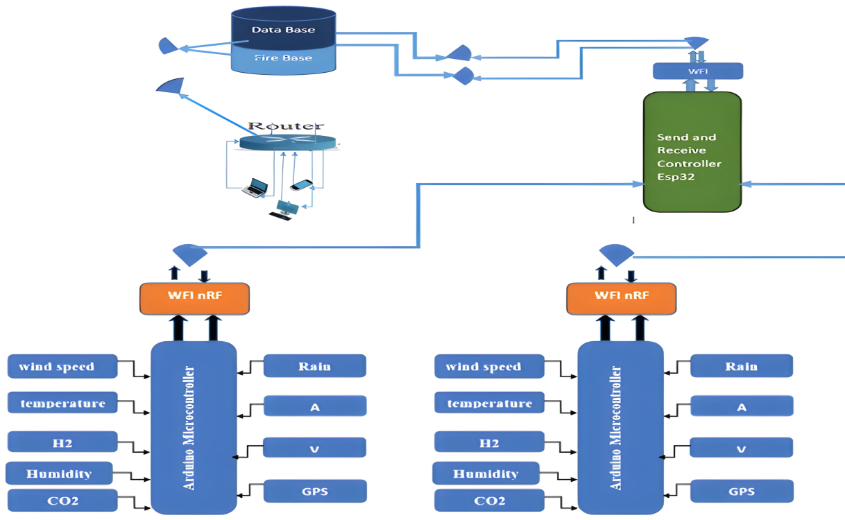
Fig. 3. Shows the structure of the system.
