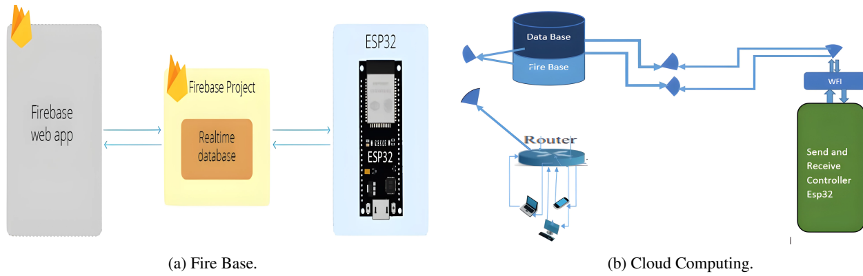
Fig. 6. Fire base and cloud computing.
