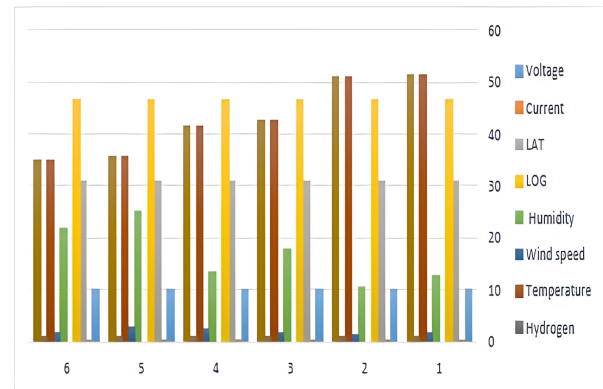
Fig. 10. Graph of the climatic values of the Euphrates River obtained at 9 am, 5 pm, and 9 pm. Node1, Node2.
