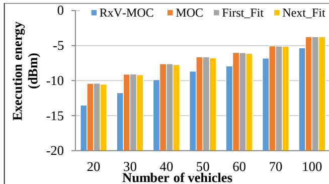
Fig. 10: Execution energy consumption.
