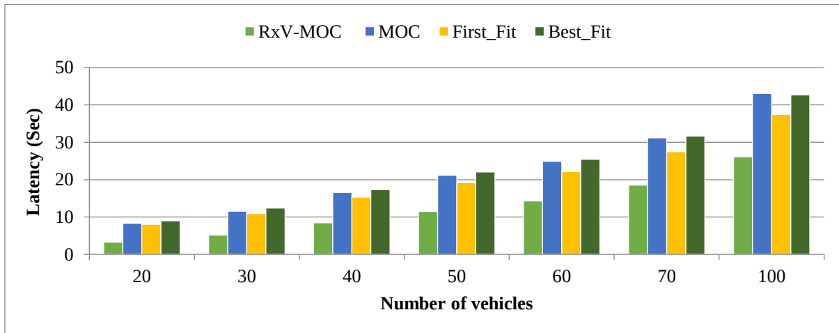
Fig. 2: Comparison of the average latency of RxV-MOC, MOC, First-Fit, and Best-Fit versus the number of vehicles.
