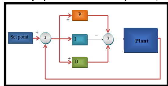
Fig. 2: PID control system.
