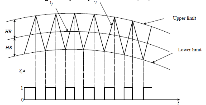
Fig. 5: Hysteresis control principle [14].
