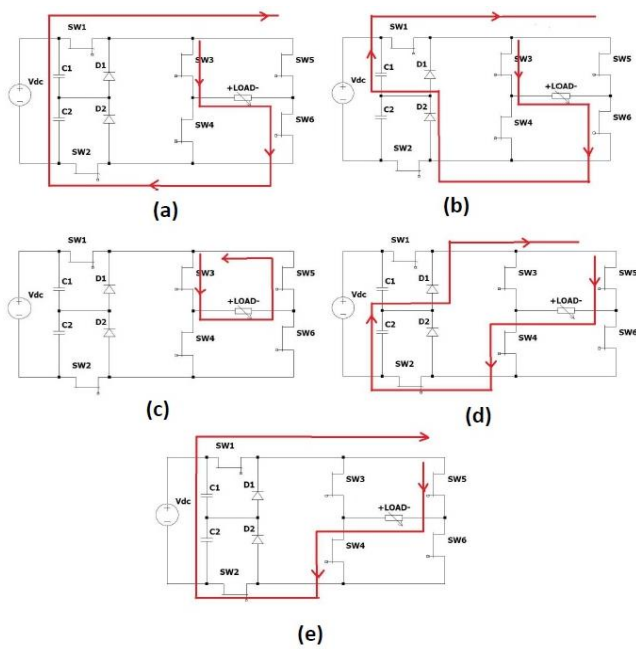
Fig.5: Operation modes of proposed five-level inverter (a) Mode 1 ( V_{out}=+V_{dc} ) (b) Mode 2 ( V_{out}=+1/2V_{dc} ) Mode 3 ( V_{out}= 0 ) (d) Mode 4 ( V_{out}=-1/2V_{dc} ) (e) Mode 5 ( V_{out}= -V_{dc} ).
