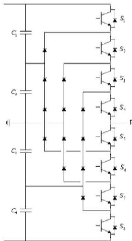
Fig. 1: Structure of diode clamped multilevel inverter.
