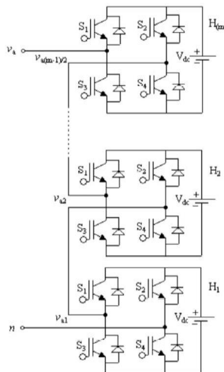
Fig. 2: Structure of cascaded multilevel inverter
