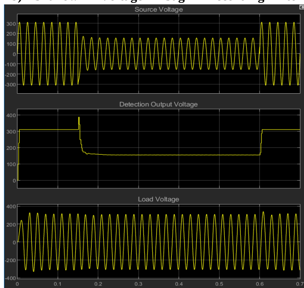
Fig. 5: Response of Numerical Matrix Detection algorithm due to 50% voltage sag.
