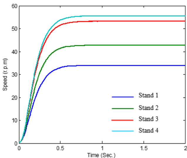
Fig.12: speed response of the work roll for each stand.
