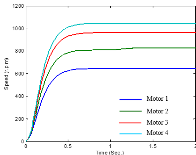
Fig.15: Motor speed responses.
