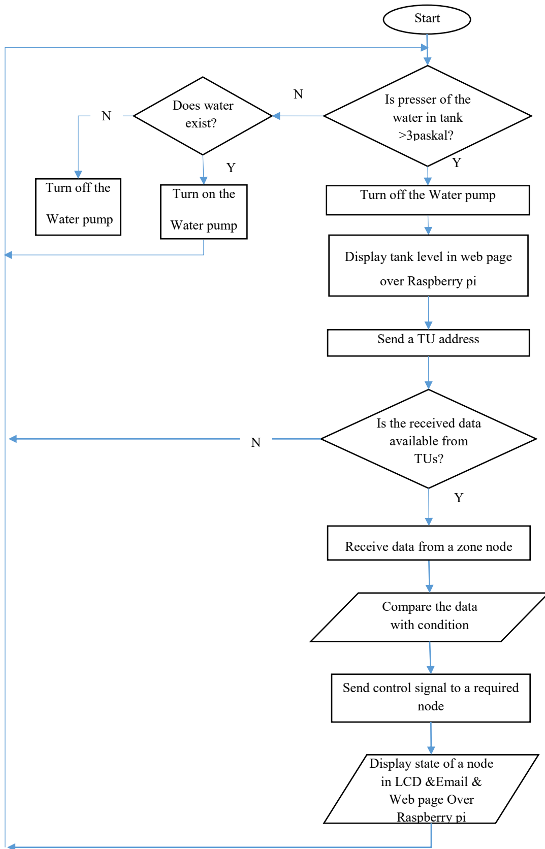
Fig. 7: (a) The BSU flowchart. (b) The TU flowchart
