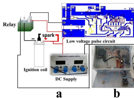
Fig. 2: (a) The circuit of high voltage pulse power supply, (b) the high voltage power supply components.
