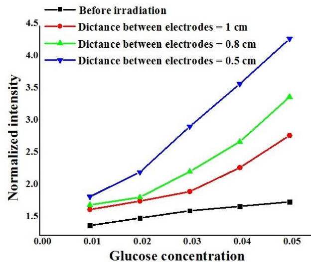
Fig. 9: Normalized intensity of the waveguide sensor versus different glucose concentrations.
