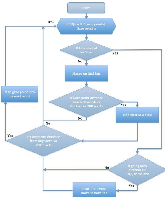
Fig. 4: Baseline algorithm flowchart.
