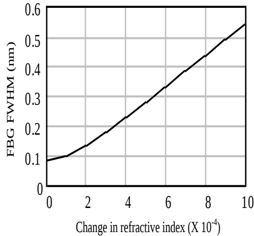
Fig. 8: Effect of \Delta n on the 3-dB spectra.
