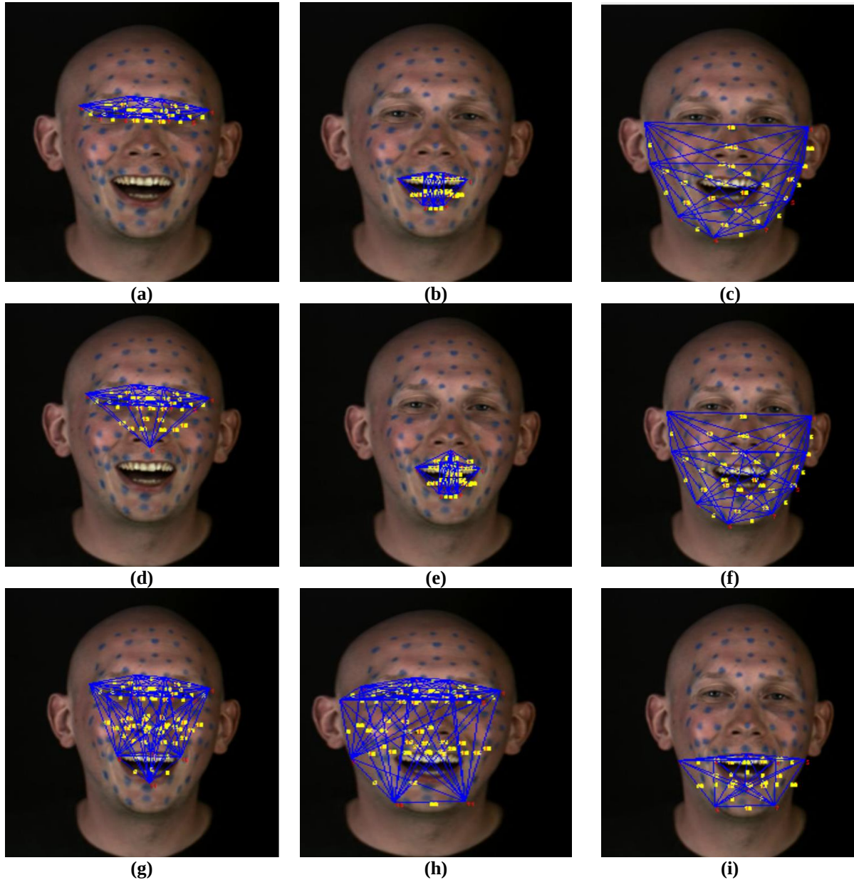
Fig. 3: Examples for the constructed graphs; (a) G_1 graph; (b) G_2 graph; (c) G_3 graph; (d) G_4 graph; (e) G_5 graph; (f) G_6 graph; (g) G_7 graph; (h) G_8 graph; (i) G_9 graph; (j) G_{10} graph; (k) G_{11} graph; (l) G_{12} graph.
