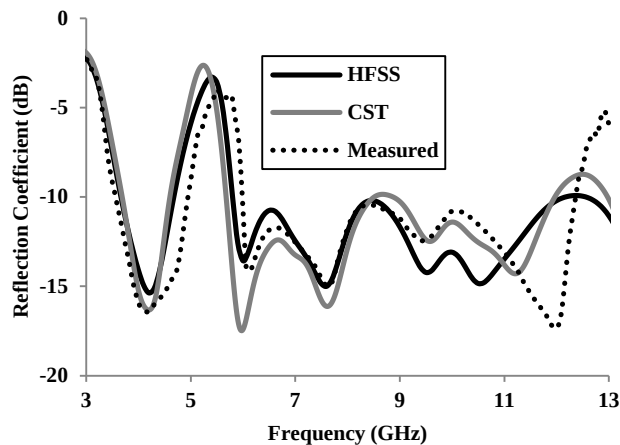
Figure 3 Comparison between the measured and simulated reflection coefficient versus frequency plots for designed antenna structure
