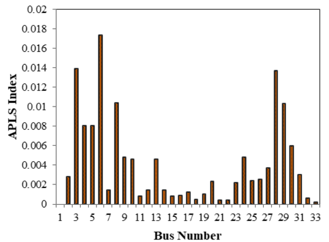
Fig. 2. APLS index for IEEE 33 bus radial PDS
