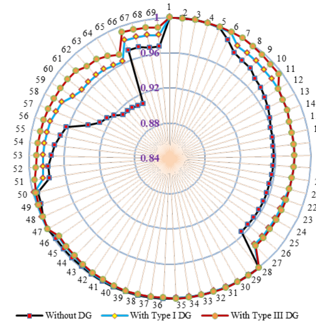
Fig. 12. Voltage magnitude of IEEE 69 bus radial PDS prior and following DG placement
