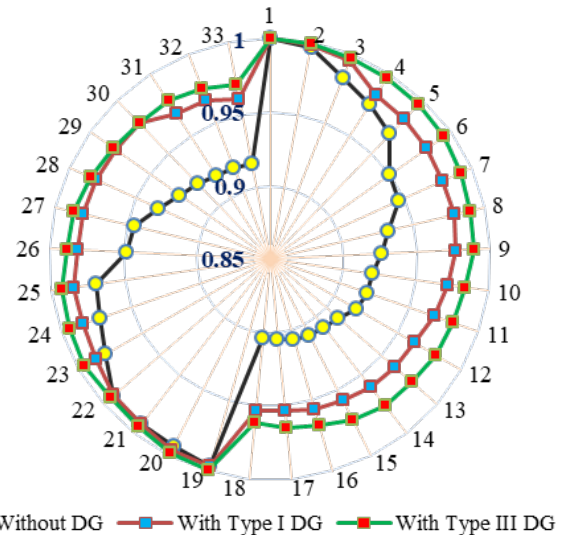
Fig. 8. BV of IEEE 33-bus radial PDS prior and following DG placement
