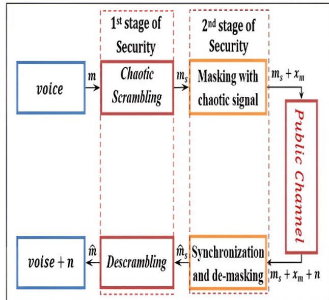
Fig. 6. Block diagram of the two chaotic levels secure proposed system, adopted from [21].
