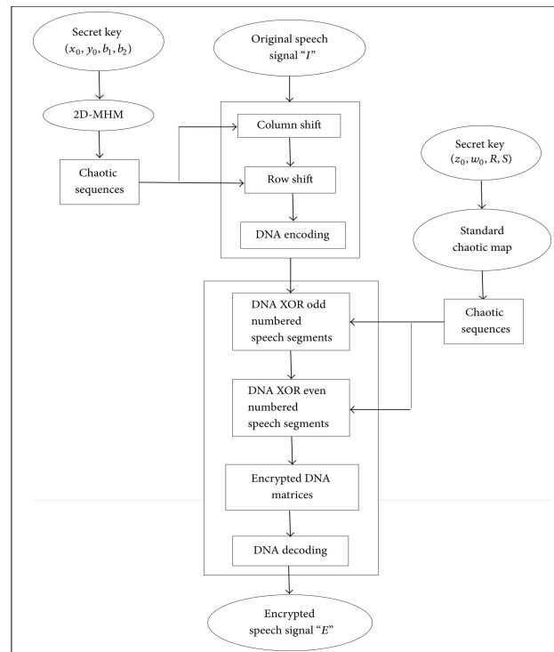
Fig. 13. Proposed encryption scheme flow diagram, adapted from [27].
