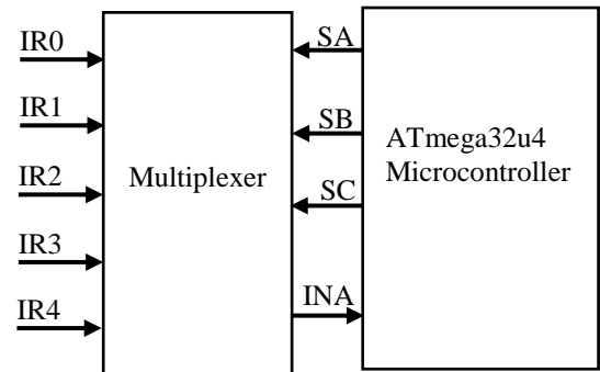
Fig. (5) the connection of the IR sensors and ATmega32u4 controller via multiplexer
