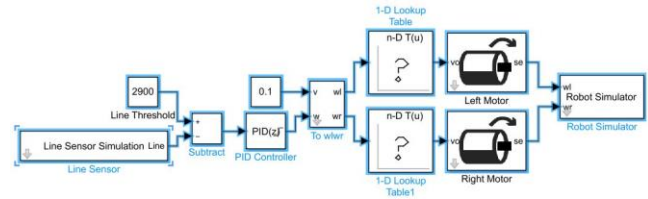
Fig. (7) Simulation block diagram of the line follower mobile robot
