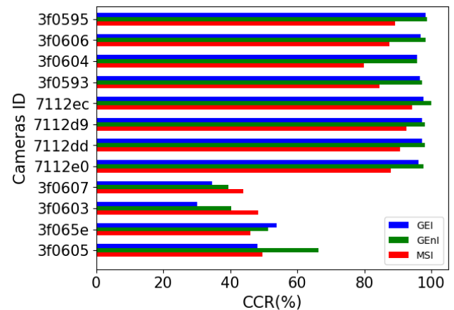
Fig. 9 Performance of different gait representations.
