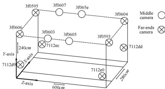
Fig. 1 The placement of the middle and far-ends synchronized cameras in the tunnel.
