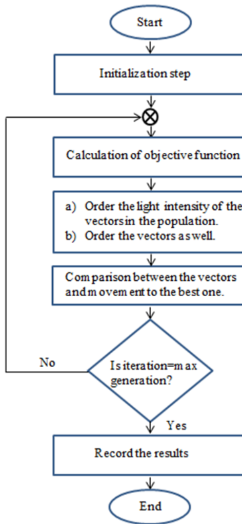
Fig. 5 Firefly flowchart
