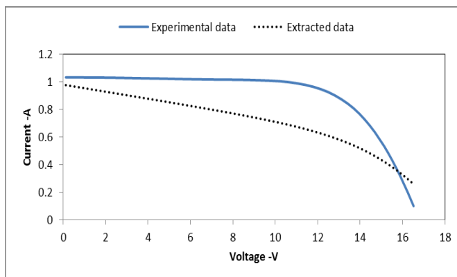
Fig. 11 Current-voltage curve using IFA for two iterations
