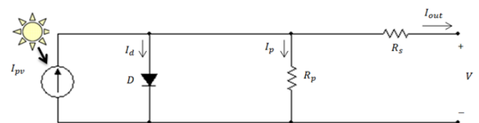
Fig. 2 Photovoltaic model
