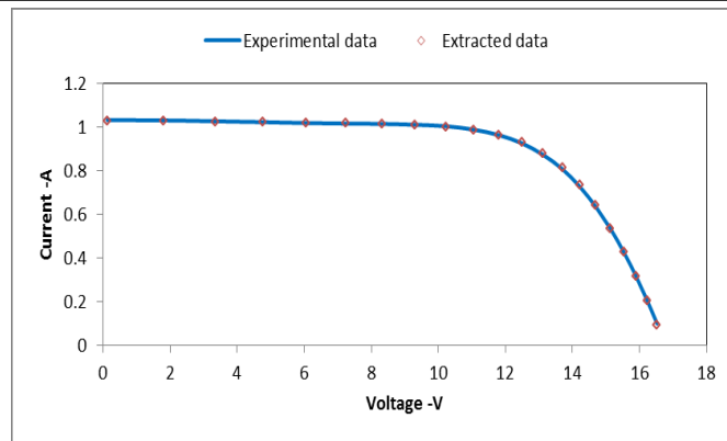
Fig. 15 Optimized Current-voltage curve using IFA
