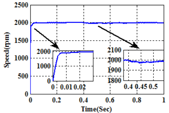
Fig.(13) Speed response under all conditions
