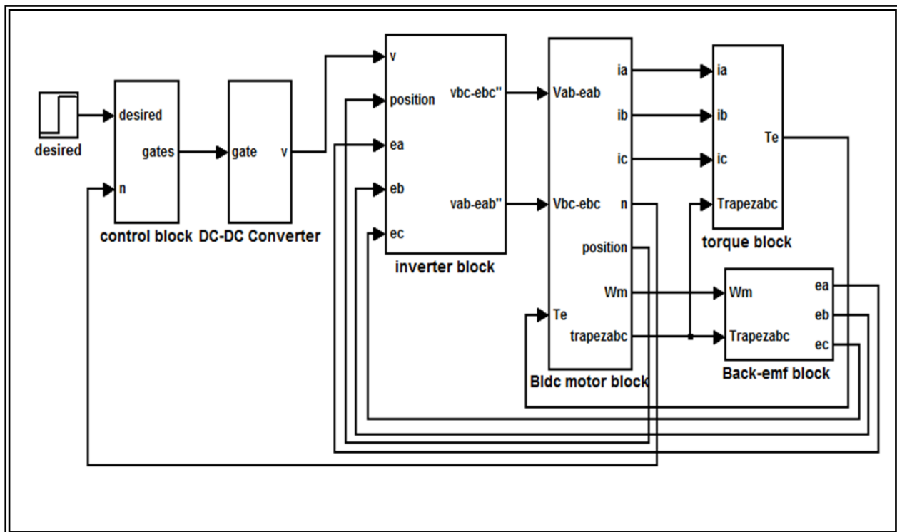
Fig.(9) Simulink model of the proposed scheme of RWNN-PID controller
