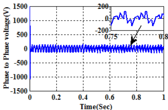
Fig.(17) Line voltage( V_{ab} ) of BLDC motor
