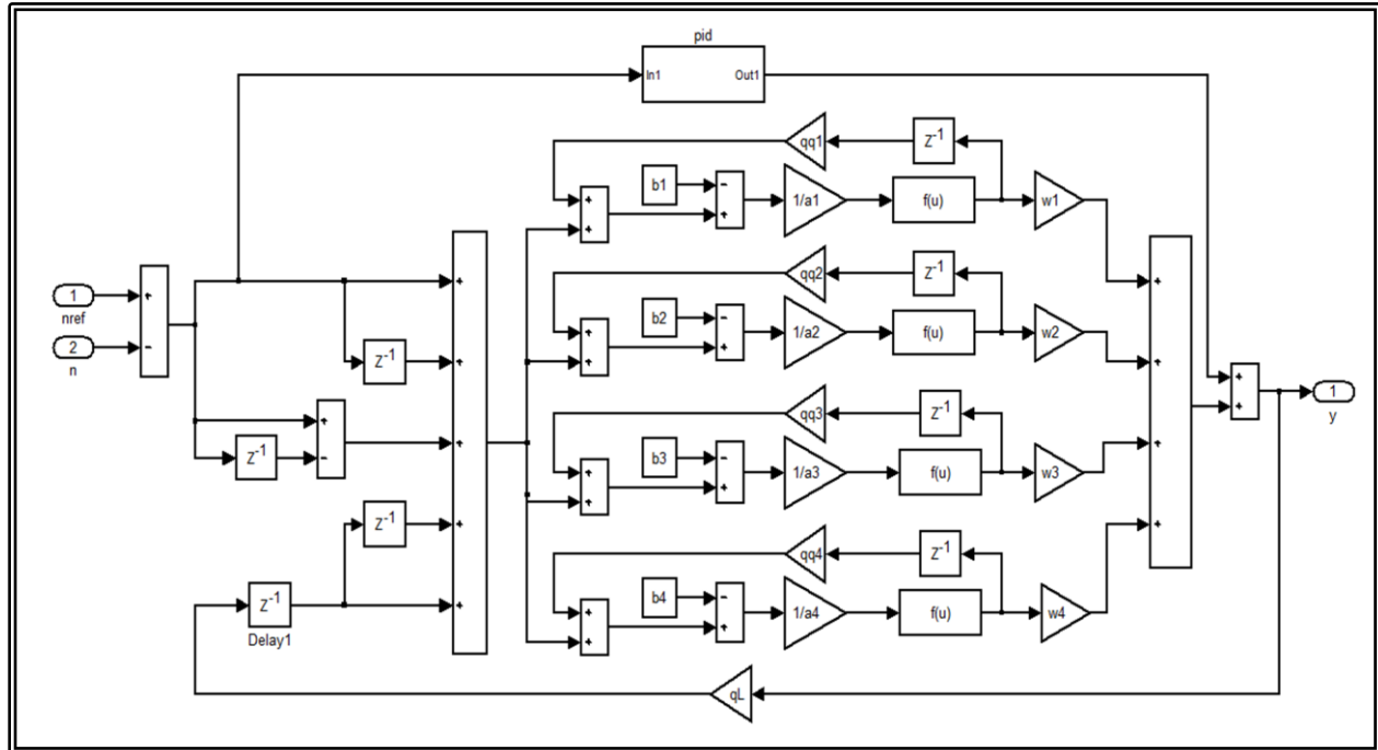
Fig.(8) Simulink model of BLDC motor drive
