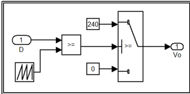
Fig.(11) Simulink model of DC-DC converter
