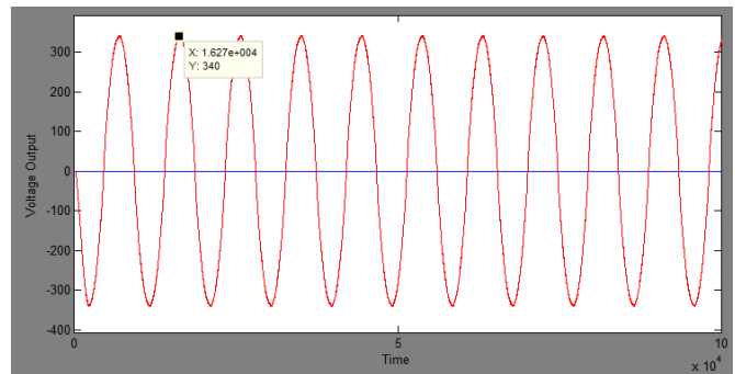
Fig. (11) Output voltage of UPS
