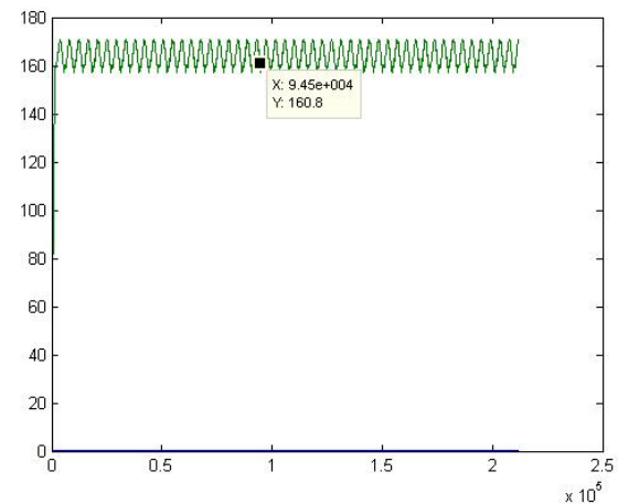
Fig. (7) Output Voltage of Rectifier before Filter
