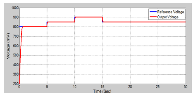
Fig.11 Matlab Simulation of Fuzzy Controller for ICCP System.
