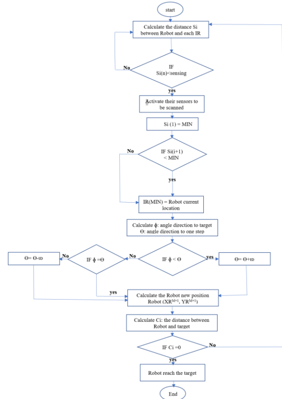
Fig. 3: The flow chart describes Shortest Orientation Algorithm
